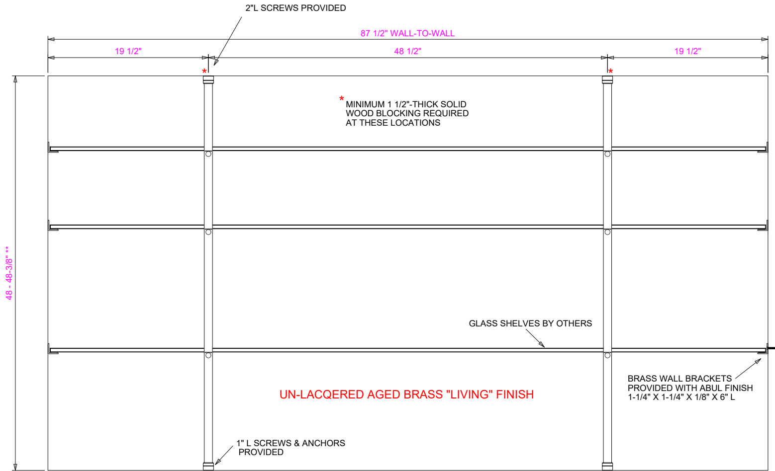
FRONT VIEW
