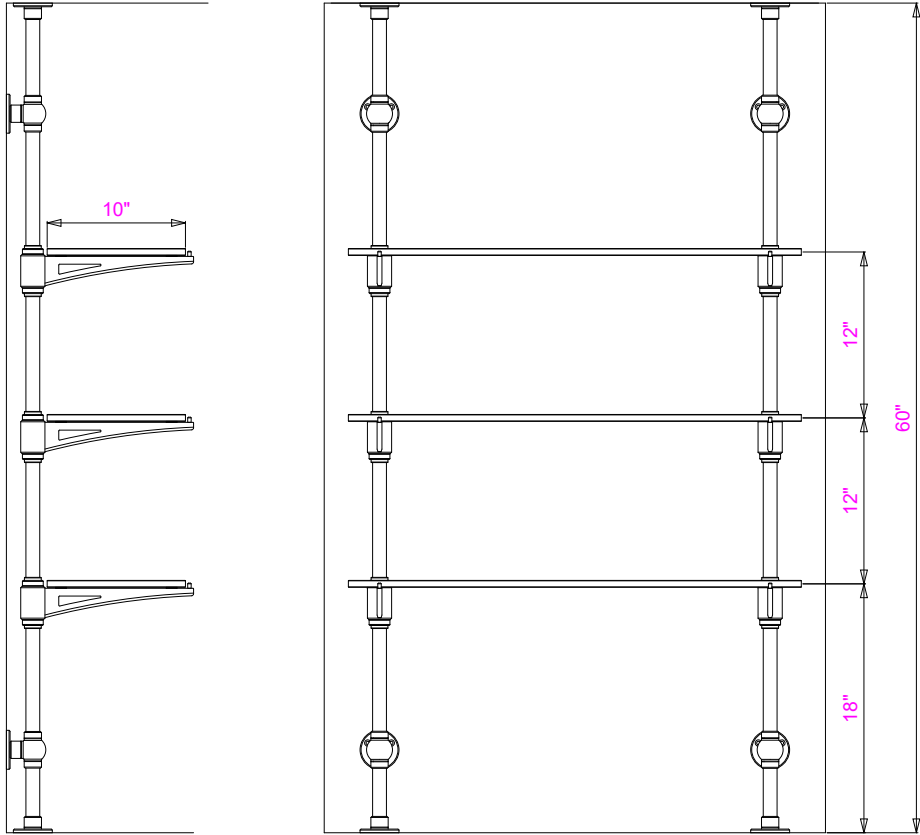
COUNTER TO CEILING OPTION
